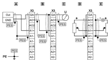
Connection of analog inputs and outputs
