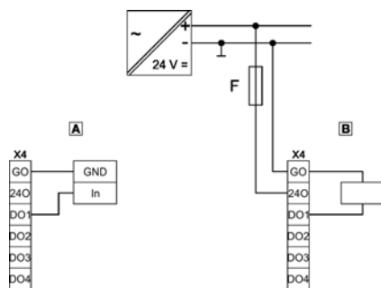
Connection of digital inputs and outputs
