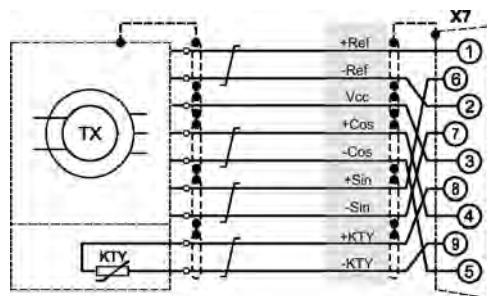
Resolver connection
