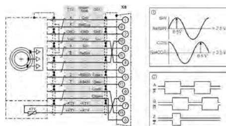
Encoder connection
