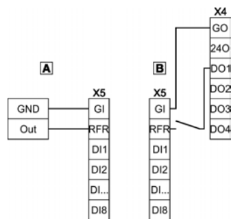
Connection of digital inputs and outputs
